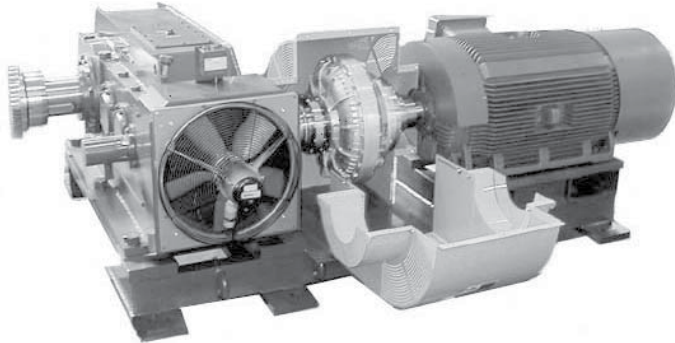
Parallel Shaft Drive & High-Speed Fluid Coupling with Type CFCG Guard
