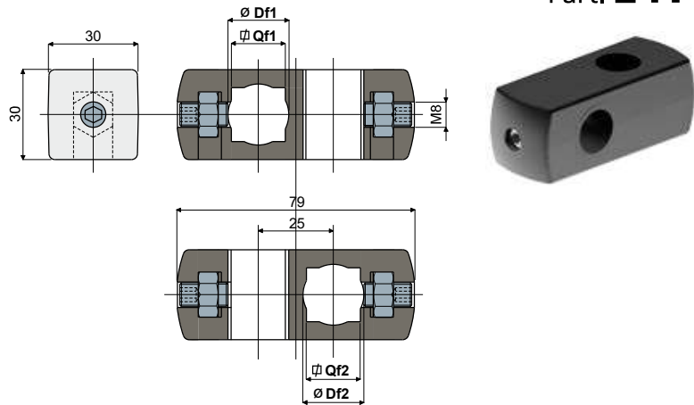
Cross clamp Part. 241
