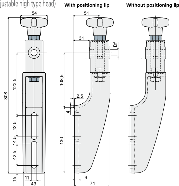
Presetting for drip tray support (see on page 29)
