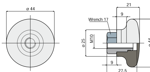
Round handle Part. 337 ( \varnothing 44 mm)
