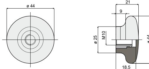
Round handle Part. 334 ( \varnothing 44 mm)
