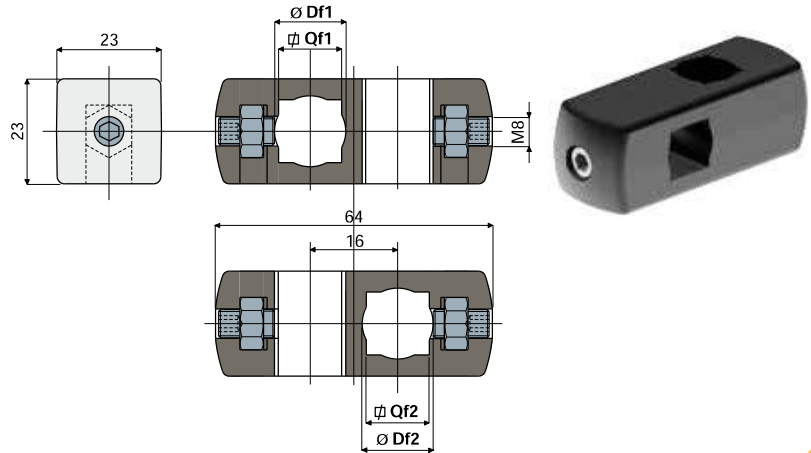
Cross clamp Part. 239
