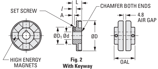
Fig. 2 Keyway Dimensions
