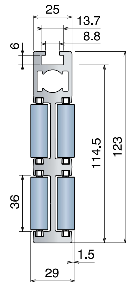
Fixing screw: M8 hex.head or PART 362 Pag 493
