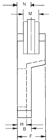
Simplex Chain
