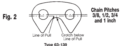
HV Chain Link Plates
