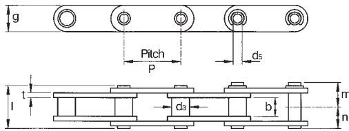
Double Pitch Rollerless Hollow Pin Chain
