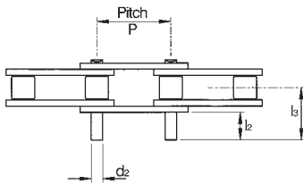
D-3 Double Pin One Side
