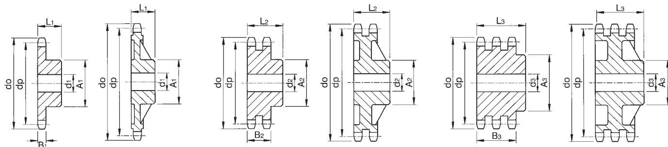
Steel Pinion
