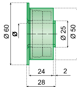
VERSION WITH FLANGE
