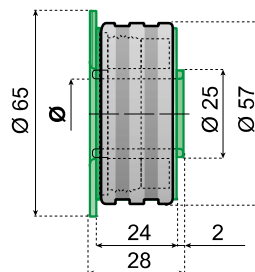
VERSION WITH FLANGE
