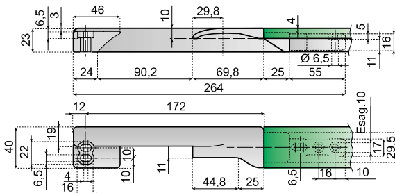
SIDE TRANSFER GUIDE SHOE - LEFT VERSION
