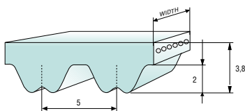
TOOTH PROFILE ACCORDING TO ISO 13050
